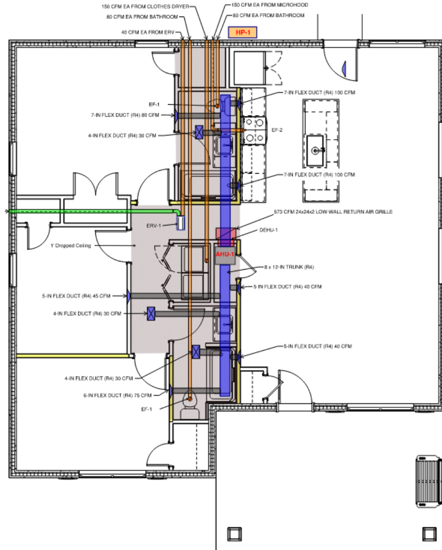
FIRST FLOOR MECH PLAN
