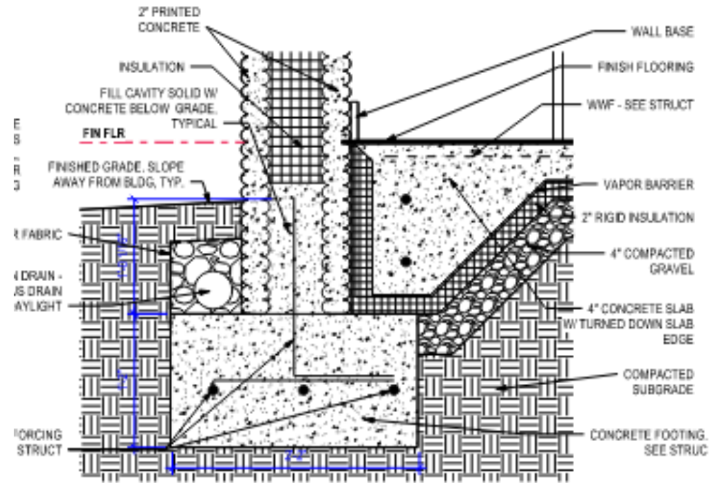
3 CONTINUOUS FOOTING DETAIL 1 1/2" = 1'-0"
